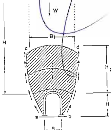
The tunnel rock-load concept of Terzaghi (1946).
